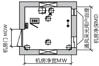
机房平面图 Machine Room Plane
