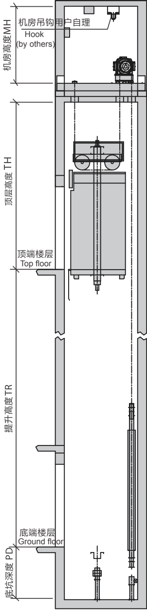
井道立面图 Shaft Vertical Section
