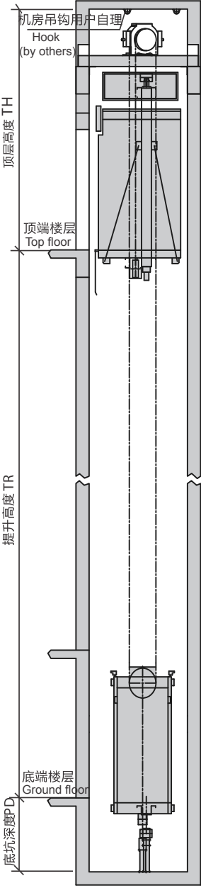
井道立面图 Shaft Vertical Section
